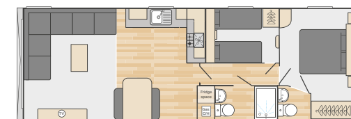
35' x 12' - 2 Bedroom
