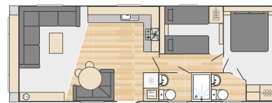
32' x 12' - 2 Bedroom
