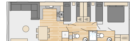
36' x 12' - 3 Bedroom
